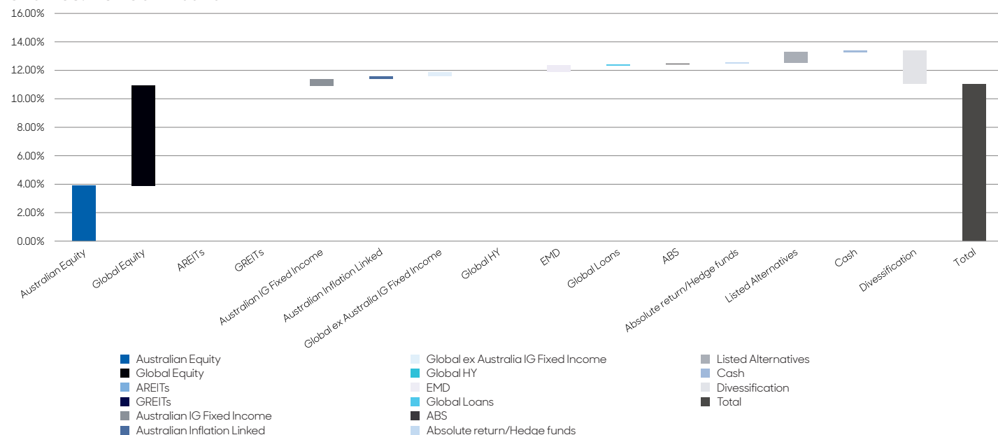
Chart 03: Risk Contribution
